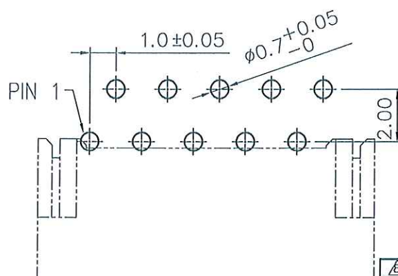
RECOMMENDED PATTERN DIM. FOR EVEN CKT. (REF.)
