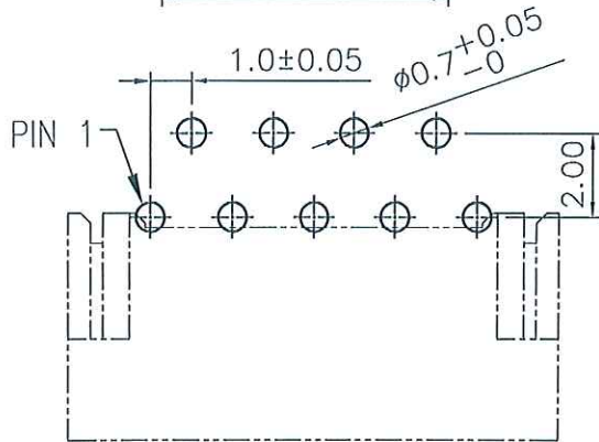
RECOMMENDED PATTERN DIM. FOR OOD CKT. (REF.)
