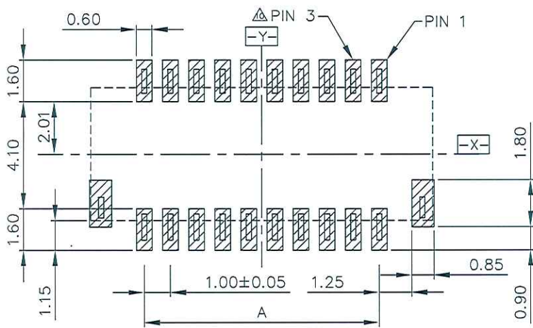
PC BOARD LAYOUT TOLERANCES: ±0.1
