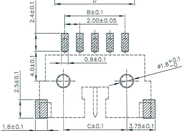
TOP VIEW RECOMMENDED P.C.B. LAYOUT
