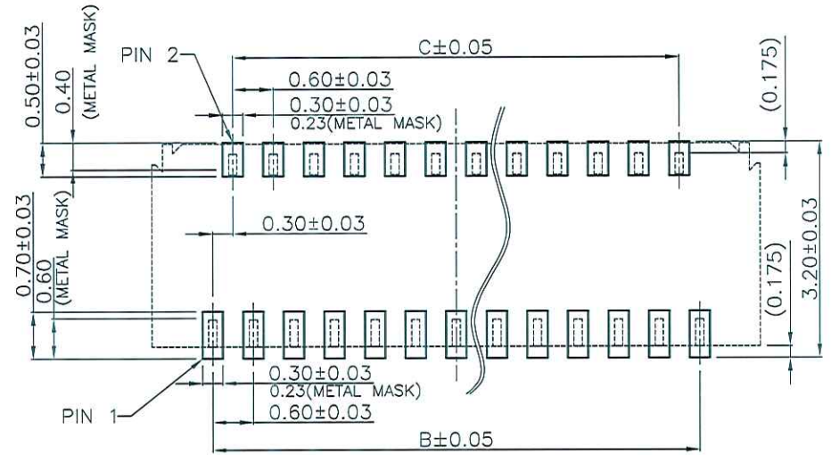
RECOMMENDED PCB MOUNTING PATTERN & METAL MASK DIMENSIONS METAL MASK THICKNESS : 0.10mm (TOP VIEW)
