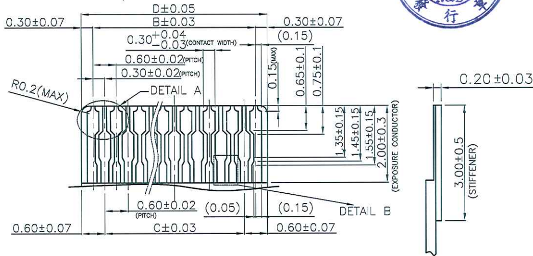
RECOMMENDED FPC DIMENSIONS
