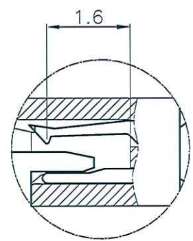
DETAIL "A" SCALE=2:1
