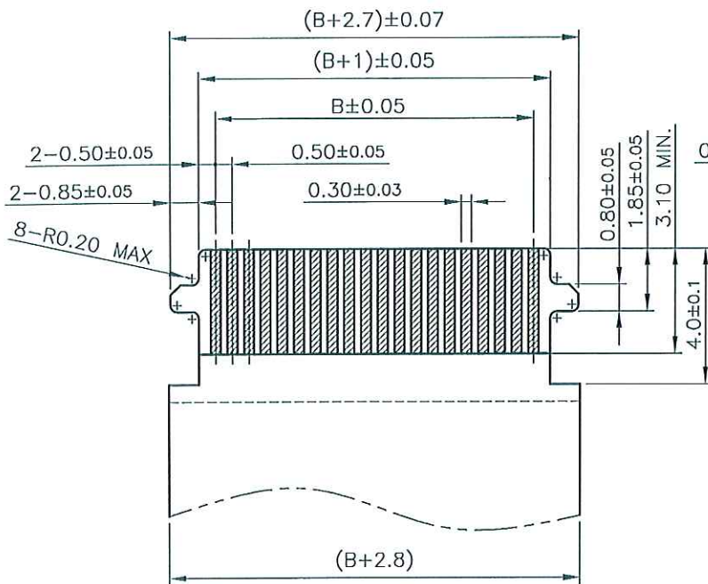
RECOMMENDED FFC DIMENSION
