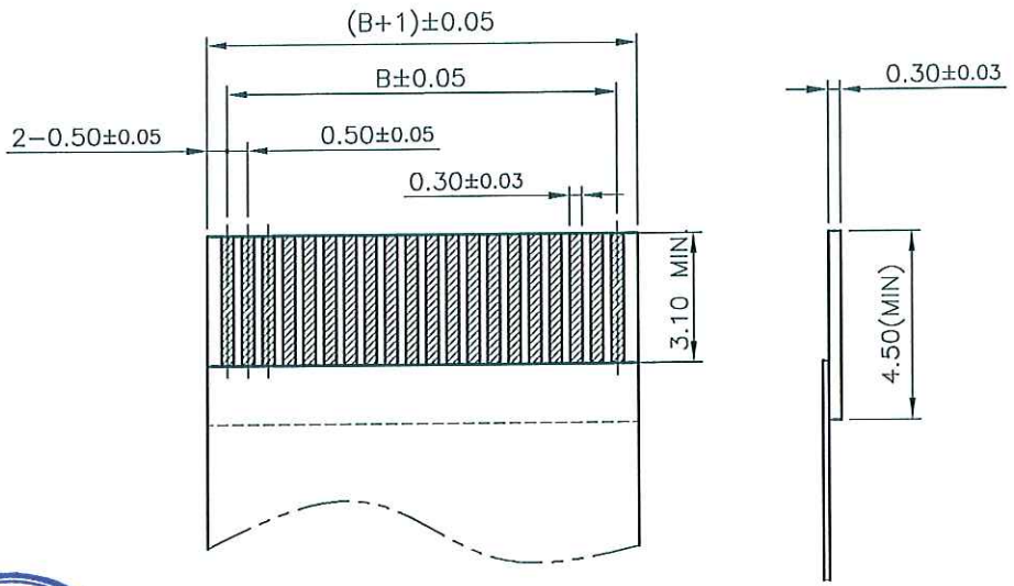
RECOMMENDED FFC DIMENSION
