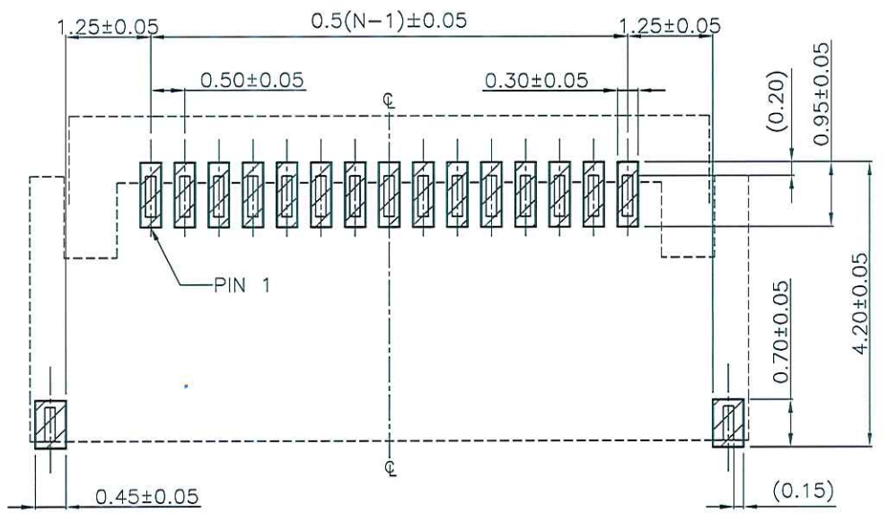
RECOMMENDED PCB MOUNTING PATTERN TOP VIEW
