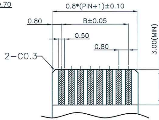
RECOMMENDED APPLICABLE FPC LAYOUT (THICKNESS: 0.3±0.03)
